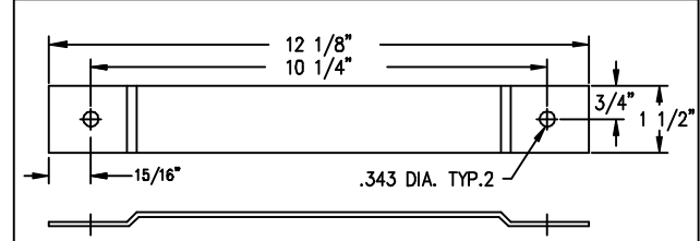
GUIDE PLATE
