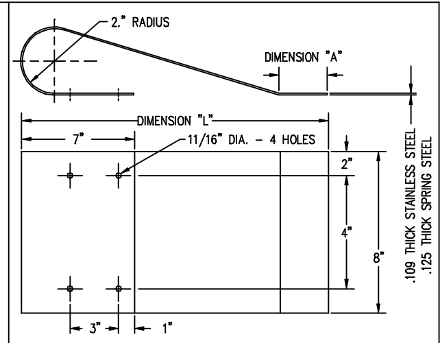
BUMPER
