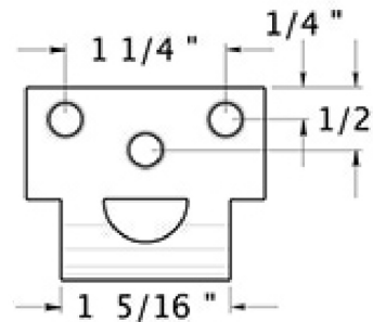
Universal Strike
