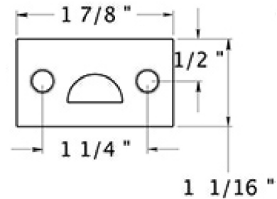
Mortise Strike
