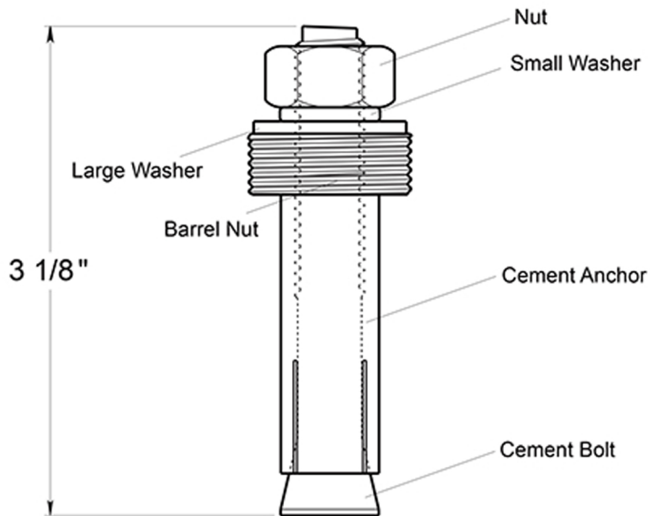
Installation Hardware
