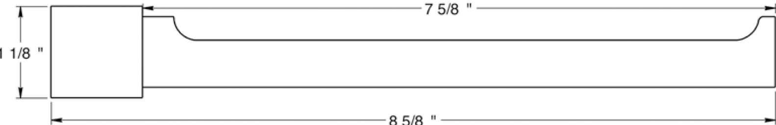
Front View
