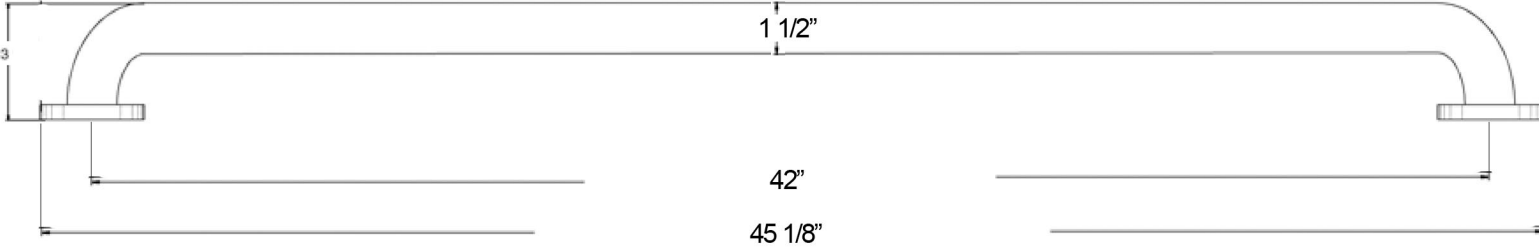
SIDE VIEW
