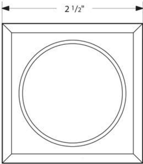
TUBULAR POCKET SQUARE ROSETTE PASSAGE, OUTSIDE TRIM
