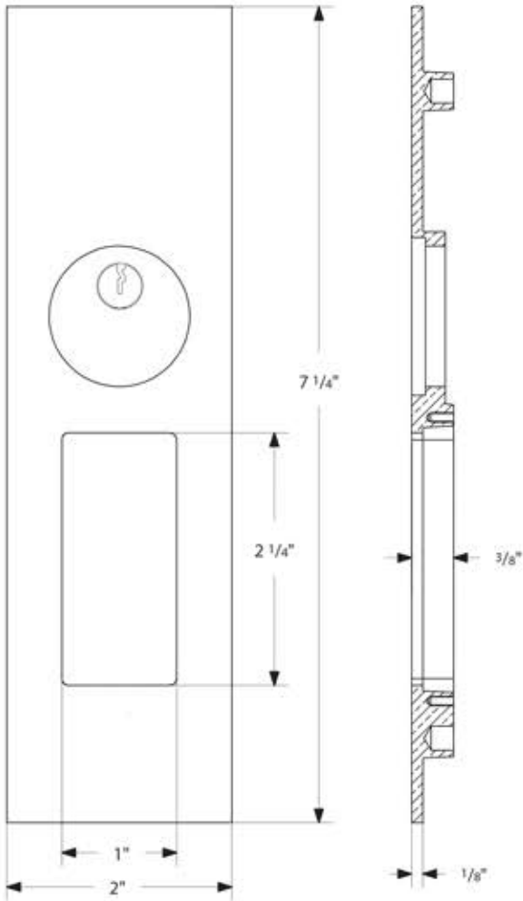
Keyed Exterior Trim
