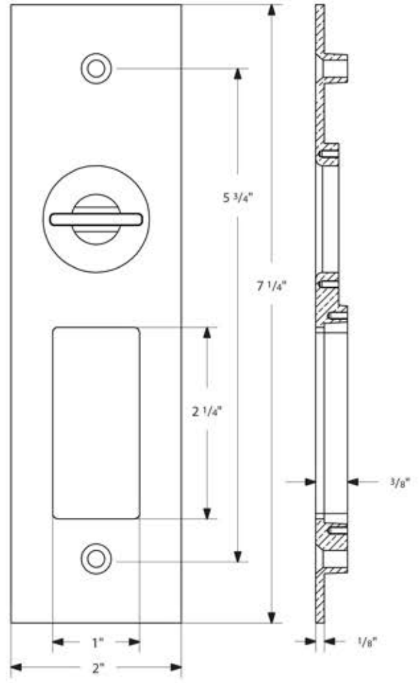
Keyed Interior Trim
