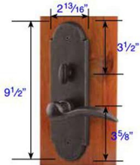
Standard interior trim Part # UL 3323
