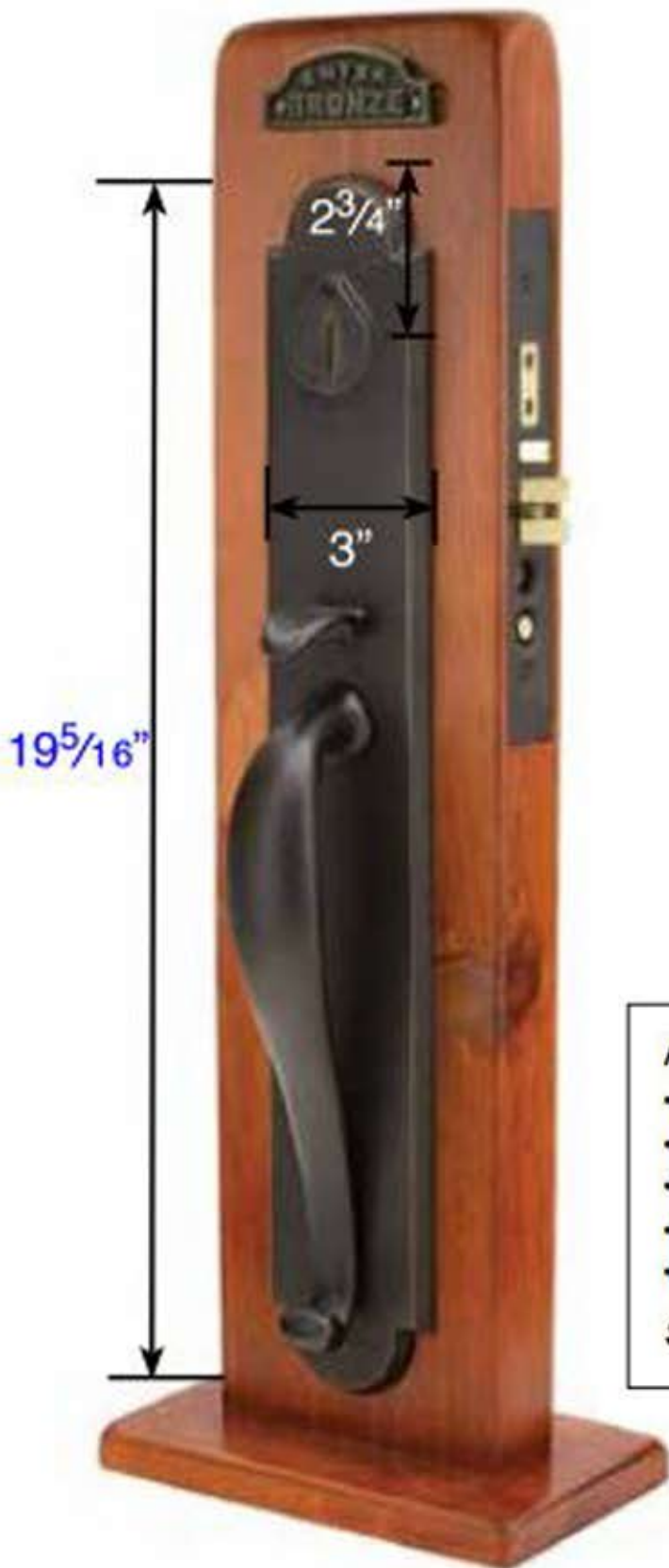
Topeka Trim Style Part # UL 3322
