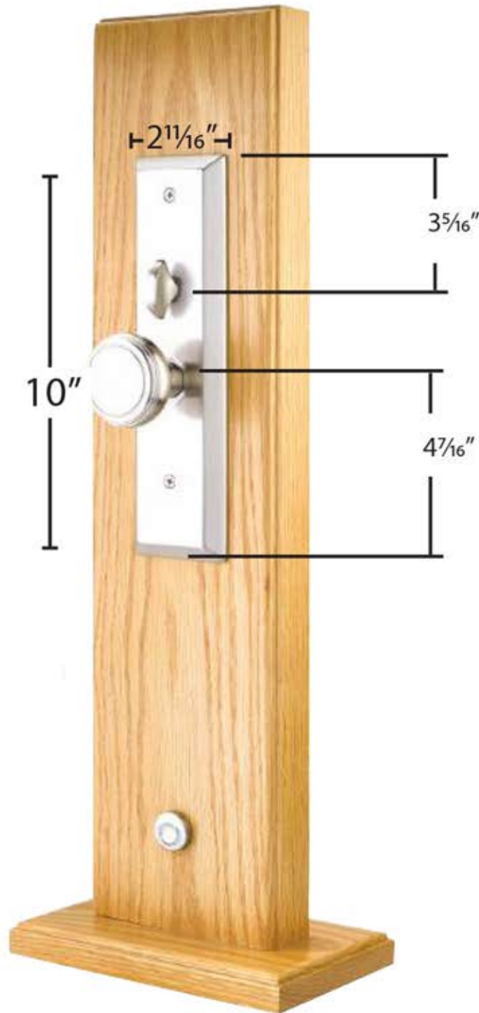
Standard interior trim Part # UL 3351 & 3352
