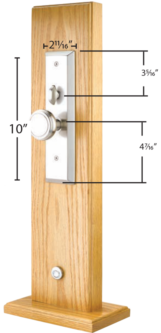
Standard interior trim Part # UL 3351 & 3352
