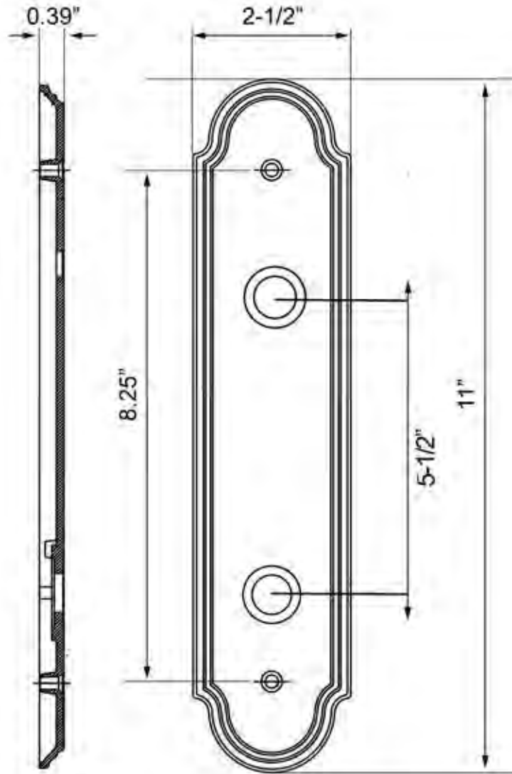
Side View
