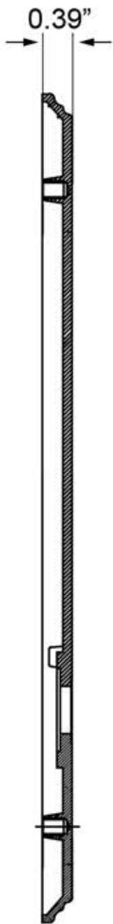
Side View
