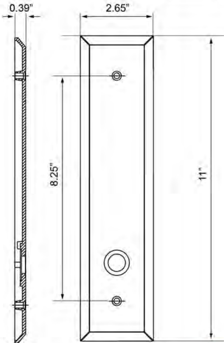
Side View
